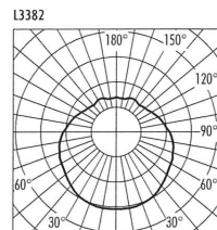
L3382 1 deling = 25 cd/1000 lm \eta_{\text{e}}: 66\% 80W HME (konv.); opal kuppel
